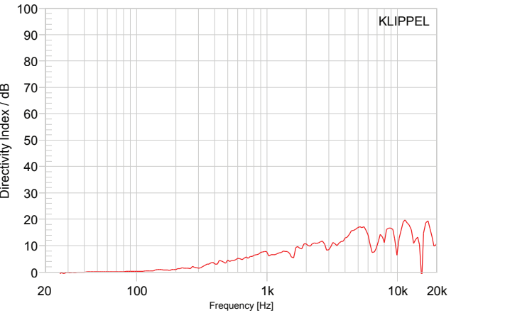
DIRECTIVITY INDEX VS FREQUENCY
